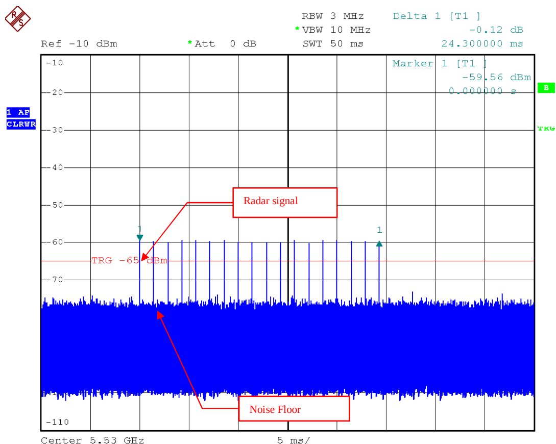
Radar Signal 1
