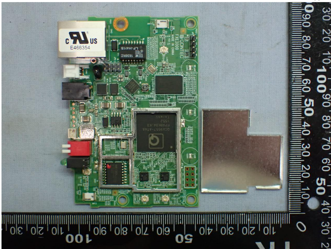
Figure 8 Internal View
