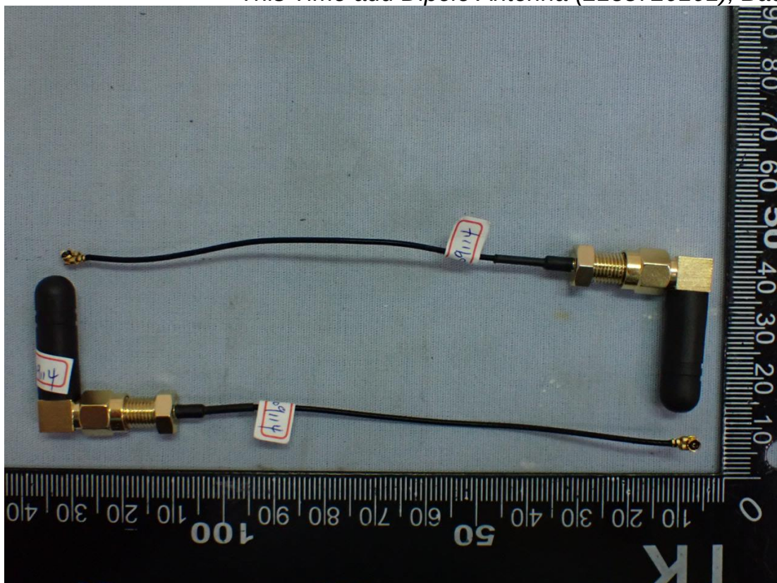
Figure 11 This Time add Dipole Antenna (2158720101), Back View
