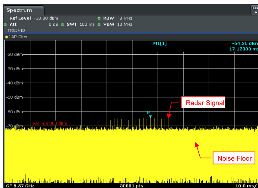
Radar Signal 0
