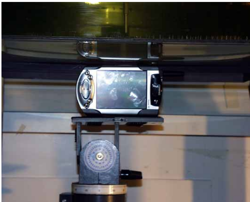
< Antenna side-face in parallel and in contact with the phantom >
