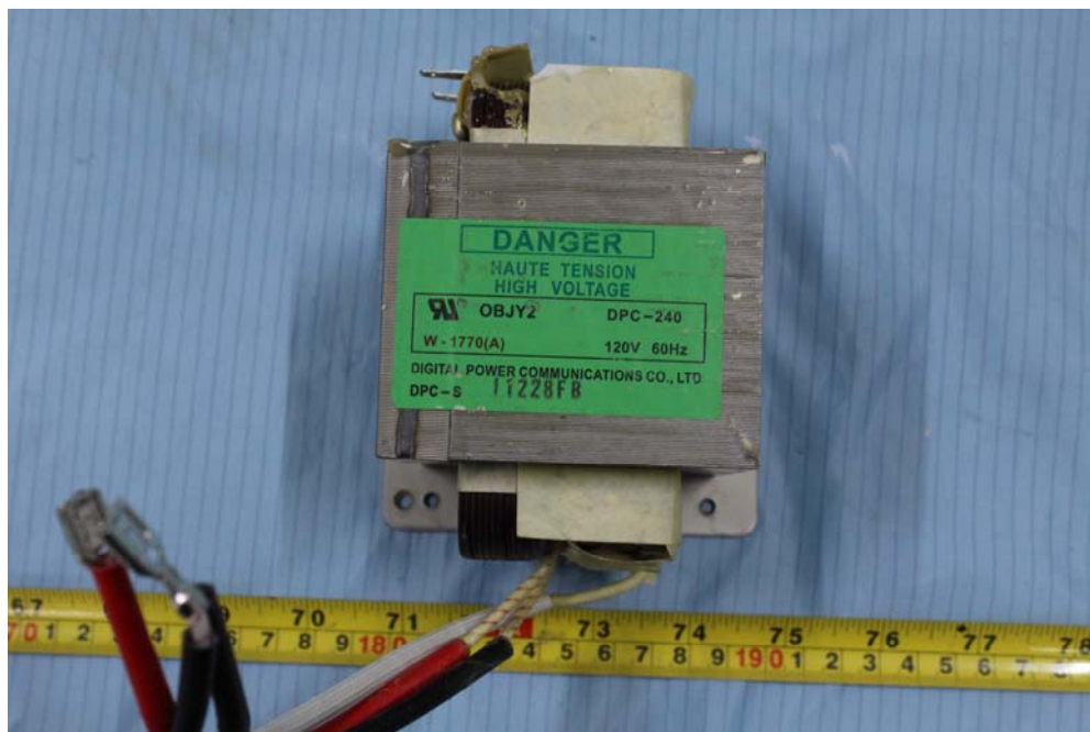
EUT –Transformer View
