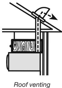
Roof venting
