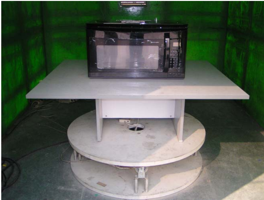
Radiated Emission–Back View
