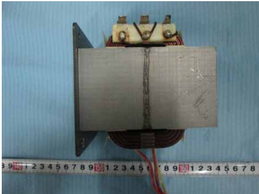
EUT – Power Transformer View
