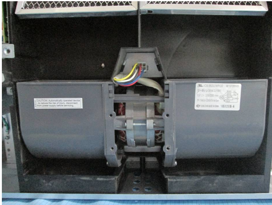
EUT – Fans 2 View
