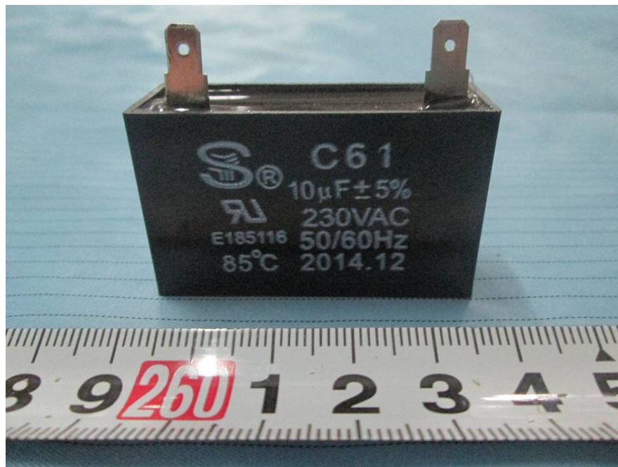
EUT – C61 View
