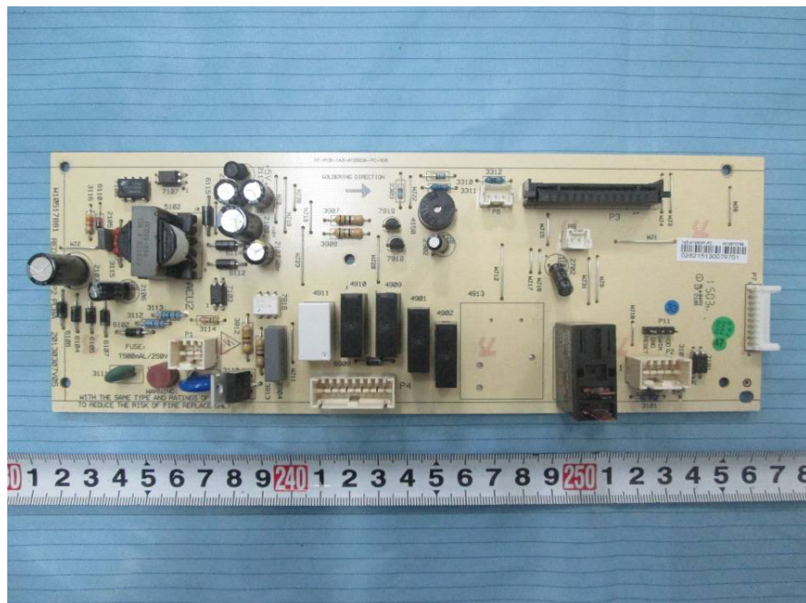
EUT – Control Pannel PCB Top View
