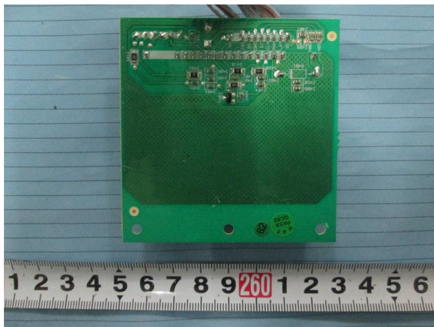
EUT – LCD Screen PCB Bottom View
