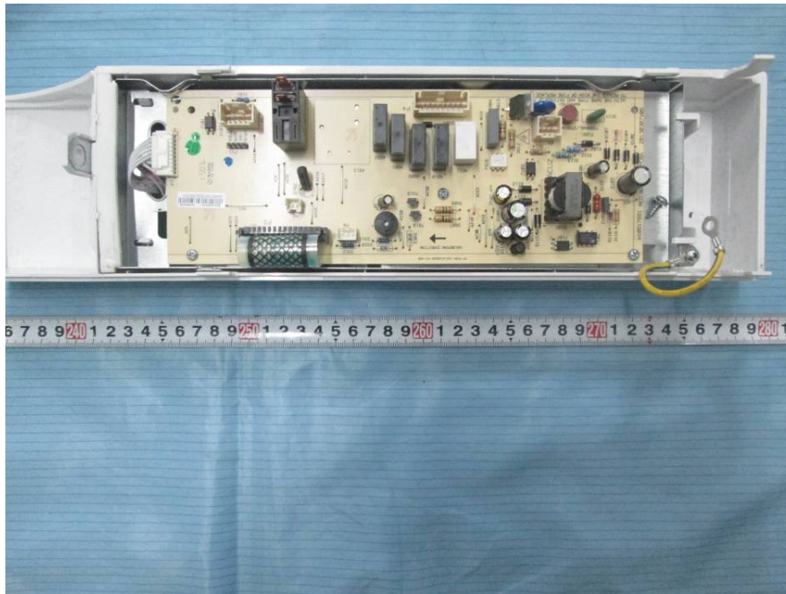
EUT – Control Pannel Rear View
