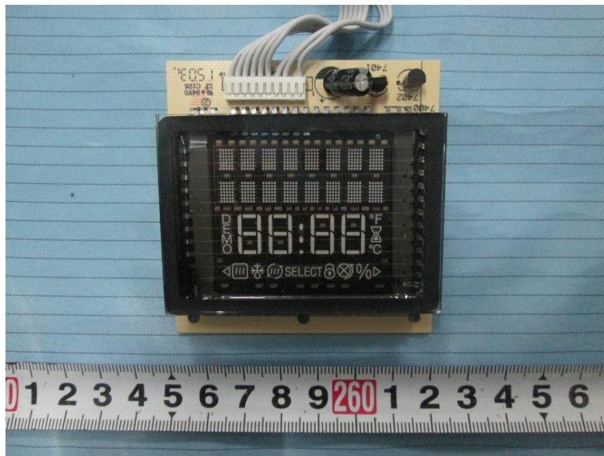
EUT – LCD Screen PCB Top View
