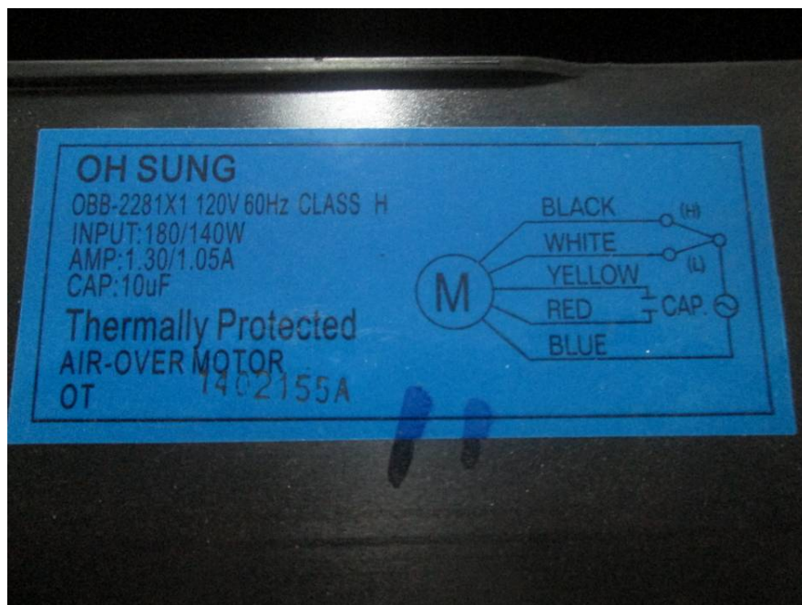
EUT – Fans Label View 1
