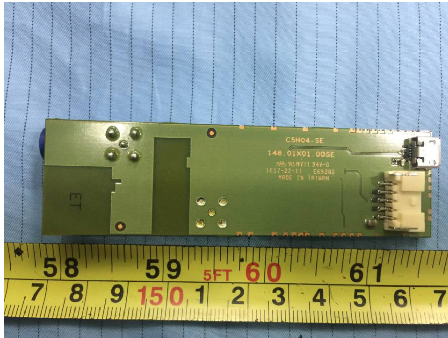
EUT – WIFI Rear View
