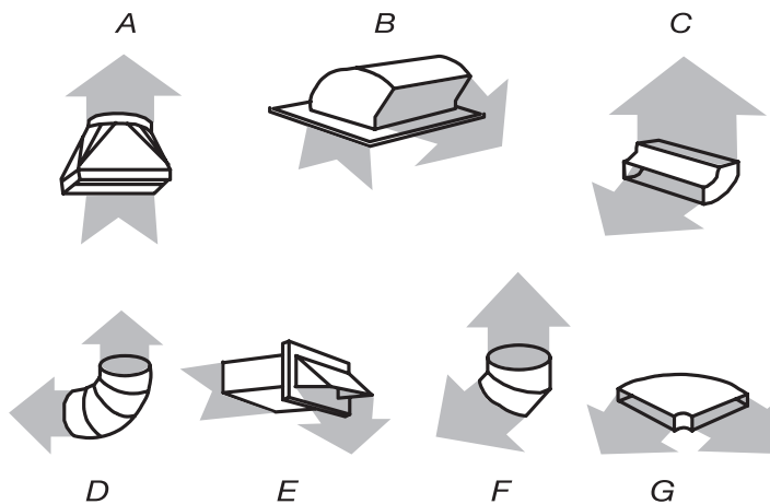
A. Rectangular-to-round transition piece: 31/4" x 10" to 6" = 5 ft (8.3 x 25.4 cm to 15.2 cm = 1.5 m)
