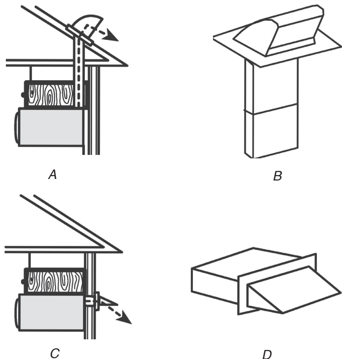
A. Roof venting
