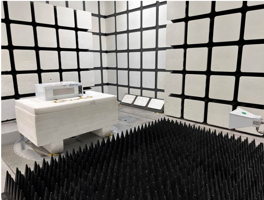
Radiated Emissions FrontView (1-18GHz)
