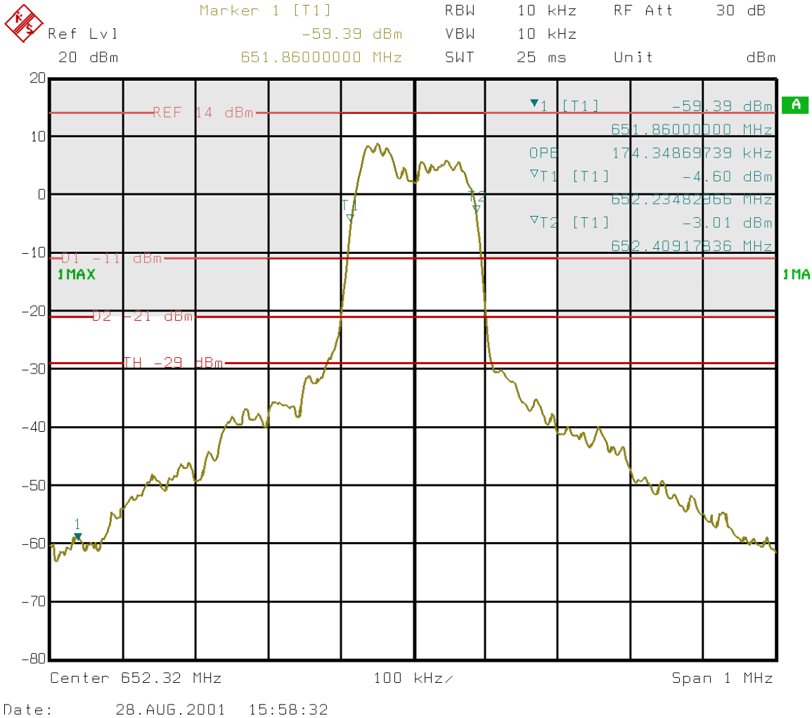
Figure 2: Occupied bandwidth spectral plot with shaded mask
