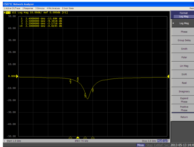
Figure 3 : Keyboard Antenna S11
