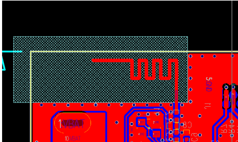
Figure 2 : Keyboard Antenna
