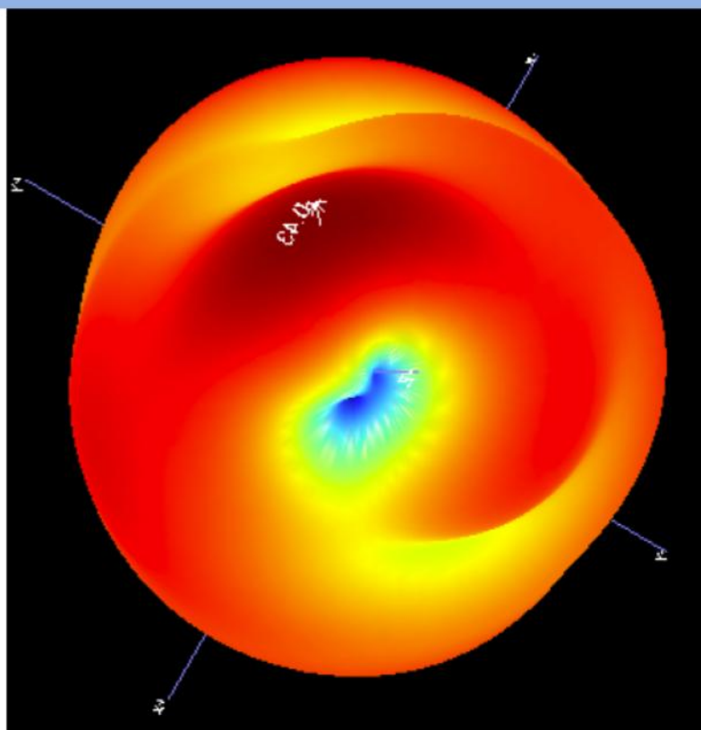
B1.3 3D Pattern for 2480MHz
