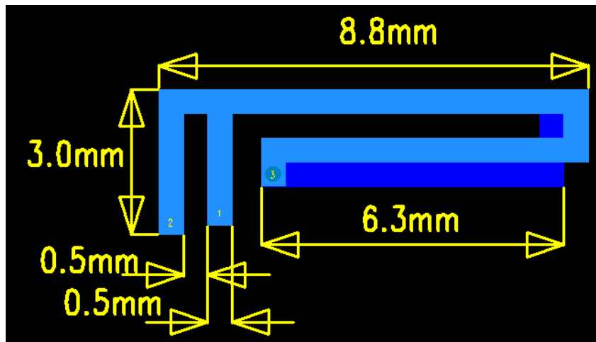
Figure 1 :Dongle Antenna
