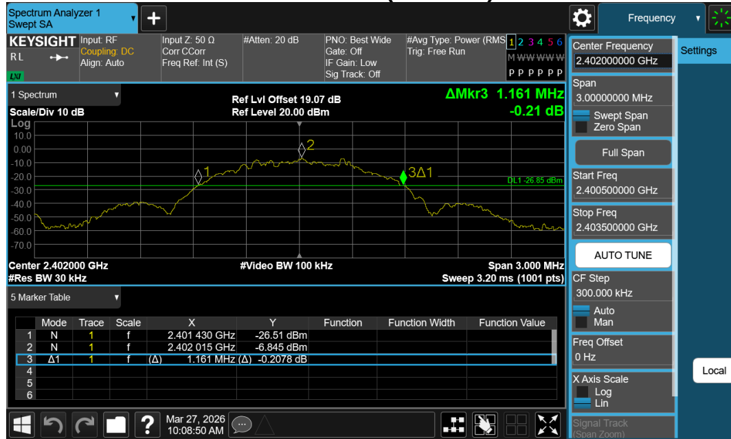
Low Channel(2402MHz)
