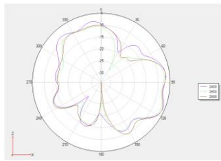
Phi 0 2D
