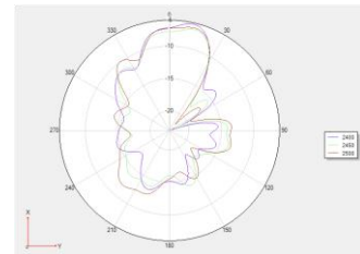
Theta 90 2D
