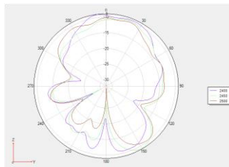
Phi 90 2D
