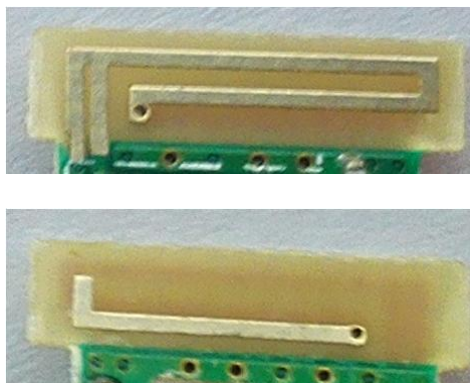
Figure 1 :Nano Dongle
