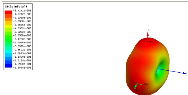
Fig.4 Nano Dongle antenna gain and 3D direction diagram (the X-axis is the left and right direction of figure 1, and the Y-axis is the upper and lower direction of figure 1)
