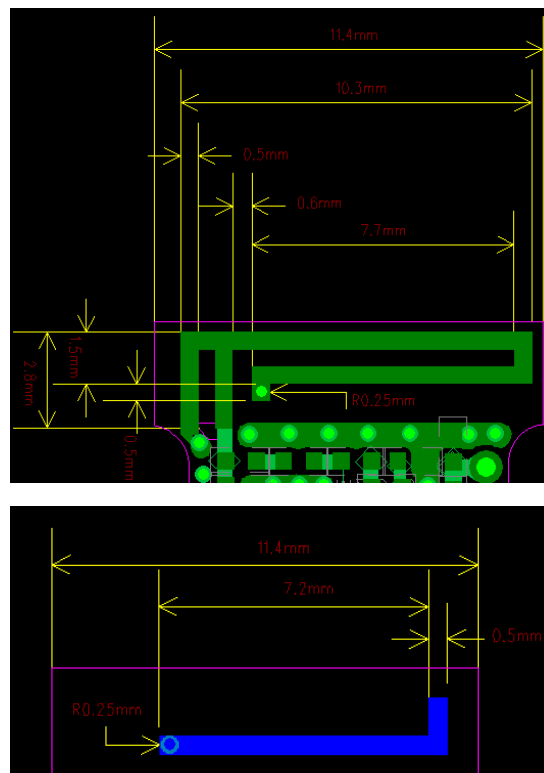
Figure 1 :Nano Dongle
