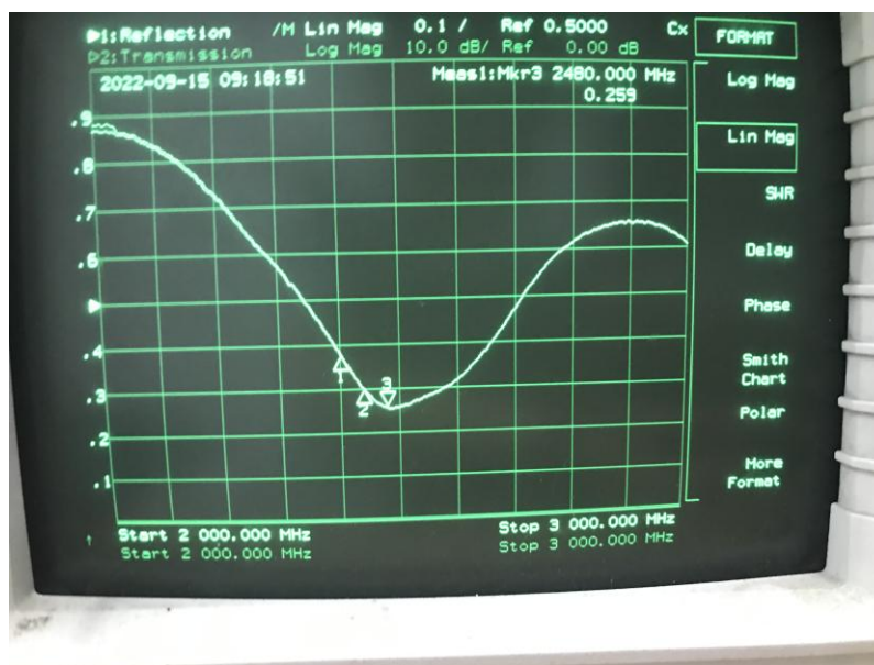
Figure 4 Dongle Antenna S11
