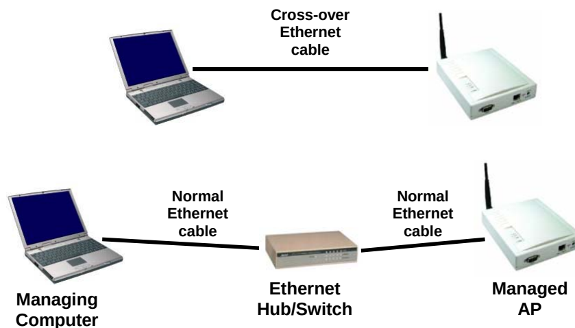
Fig. 2. Connecting a managing computer and an AP via Ethernet.
