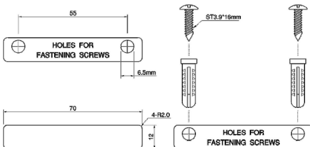
Fig. 1. Mounting the AP on a wall.
