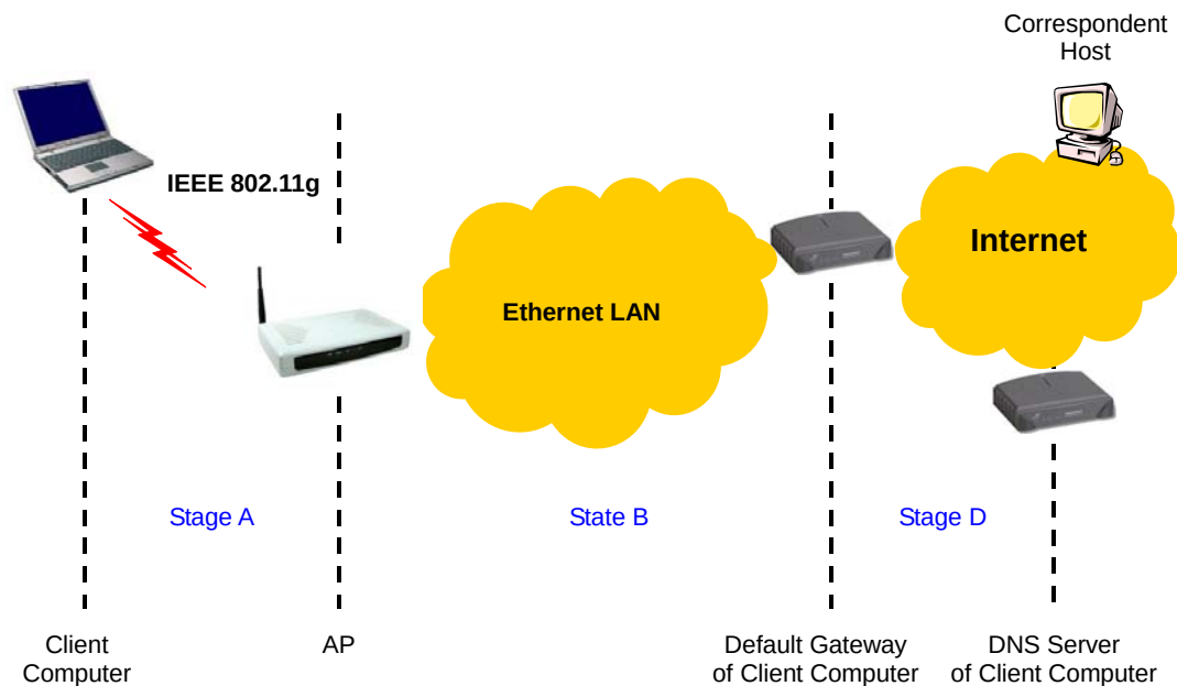
Fig. 60. Communication stages for a client to reach its correspondent host.
