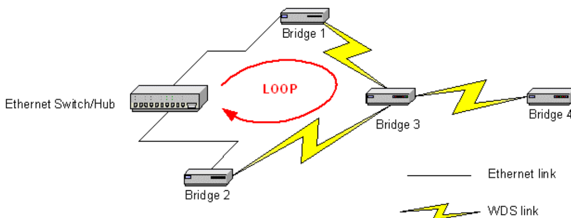
Fig. 42. Network topology containing a loop.
