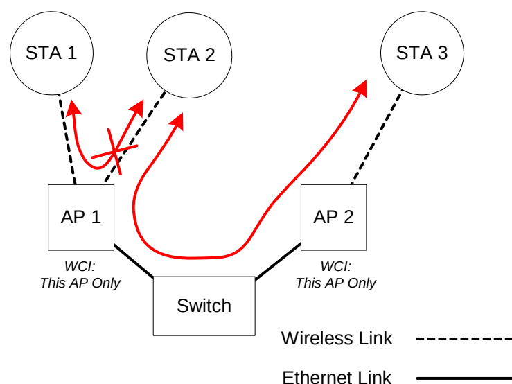
Fig. 47. Behavior of the “This AP Only” wireless client isolation option.
