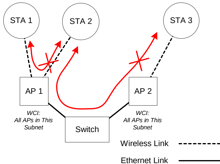
Fig. 48. Behavior of the “All APs on This Subnet” wireless client isolation option.
