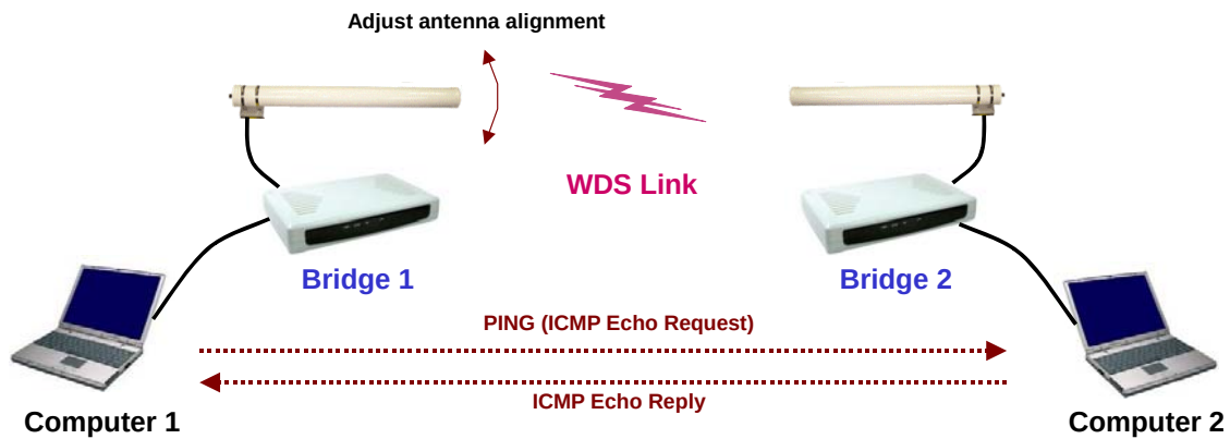
Fig. 44. Adjusting alignments of external directional antennas.
