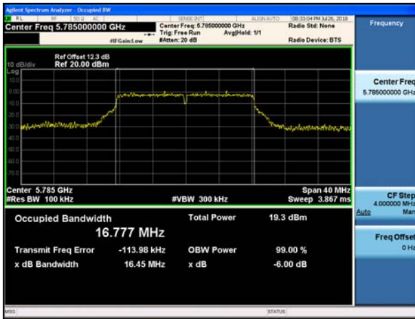
802.11a UNII 3 BAND 6dB Bandwidth (CH.157)
