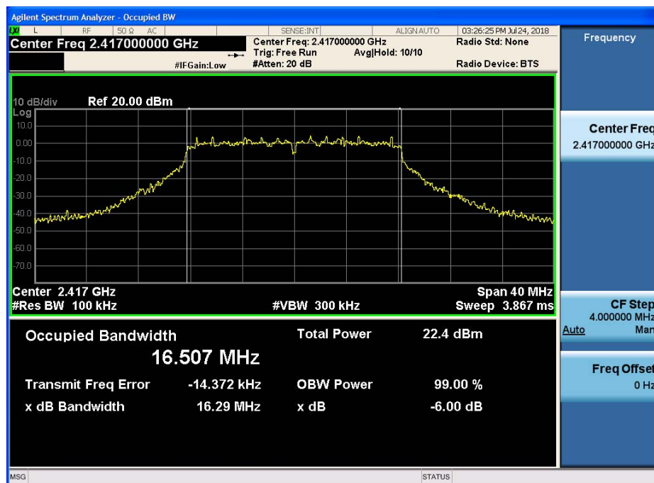
6dB Bandwidth plot (802.11g-CH 2)
