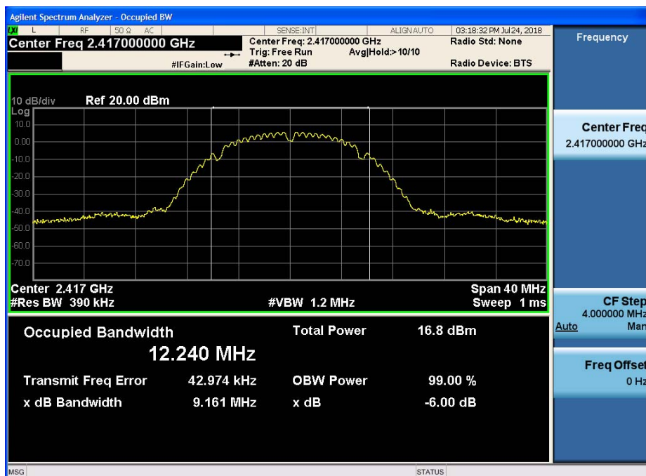
99% Bandwidth plot (802.11b - CH 2)
