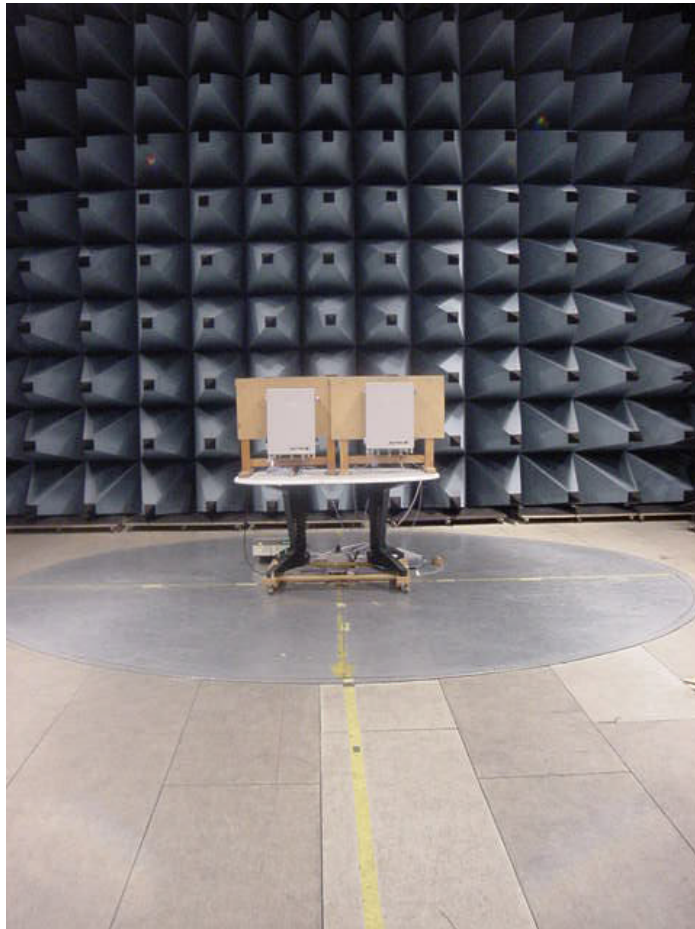
Radiated spurious emission 30 – 1000 MHz
