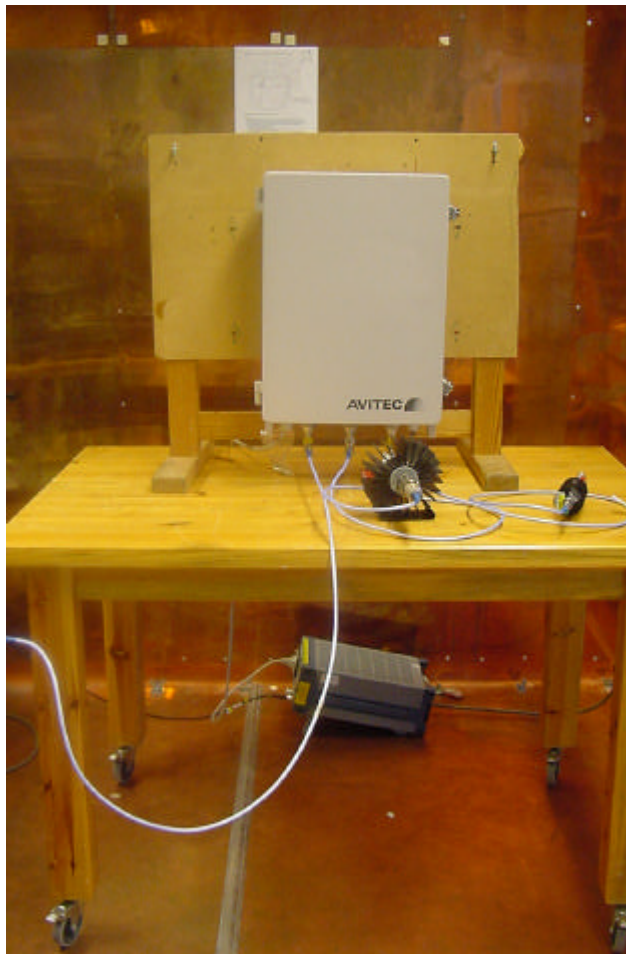
Conducted disturbance voltage in the frequency range 0,15 - 30 MHz
