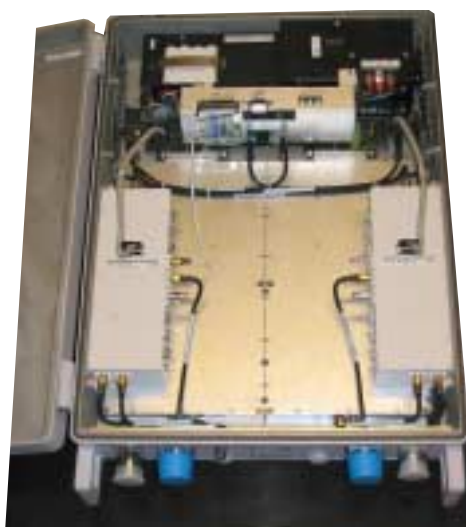
2-channel repeater
