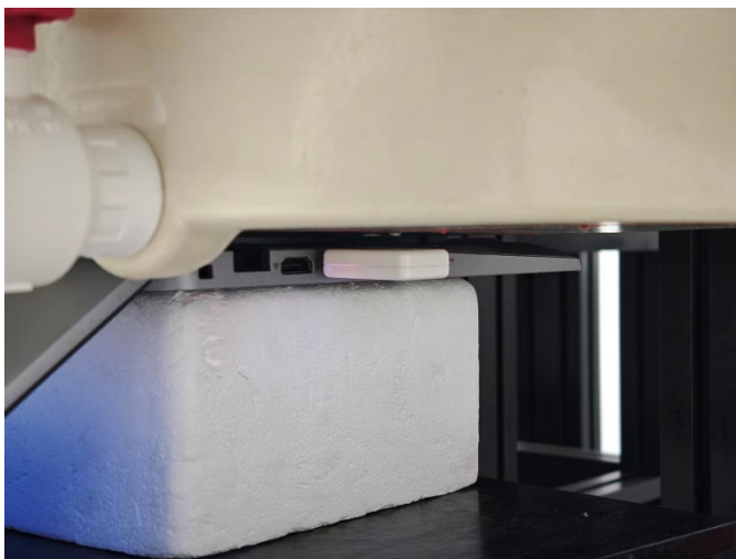
Horizontal-Up of EUT with 0.5 cm Gap (Body Mode)
