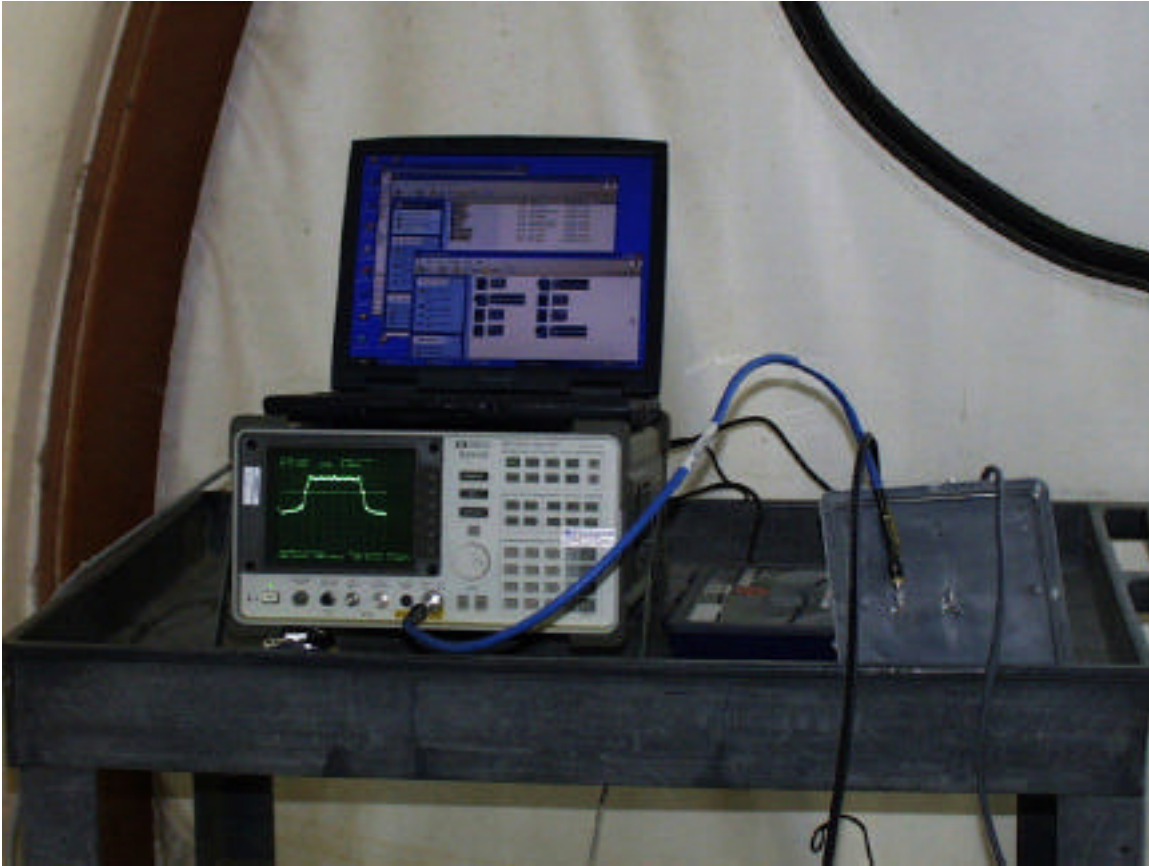
Antenna Output Conducted Measurements
