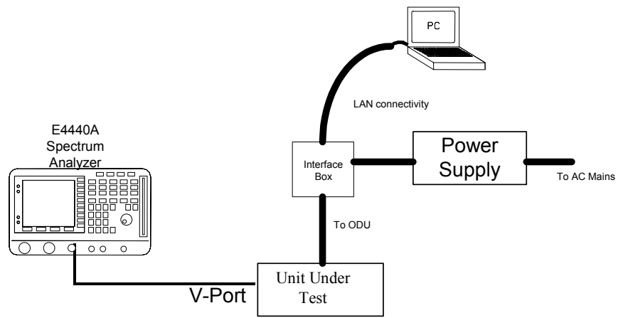
Test set-up
