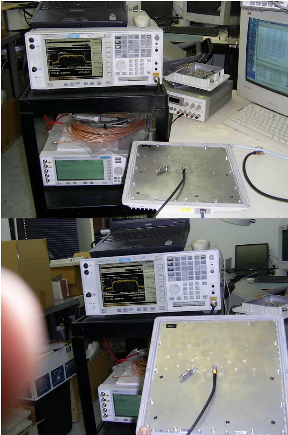
Aperto Location: Lab test set-up of Radio
