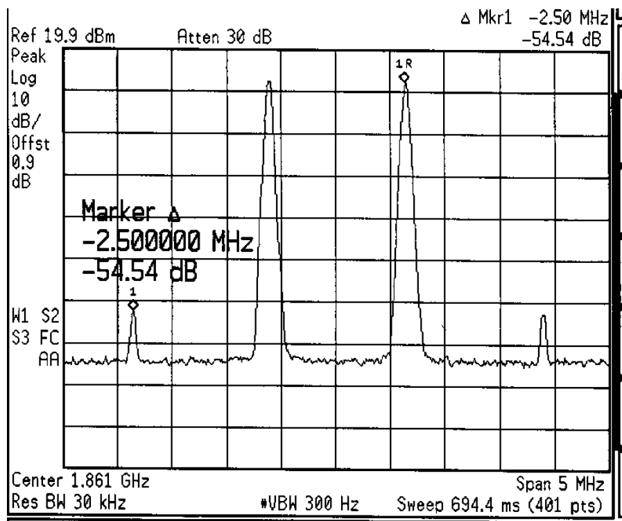
Figure 3: Intermodulation Characteristics.
