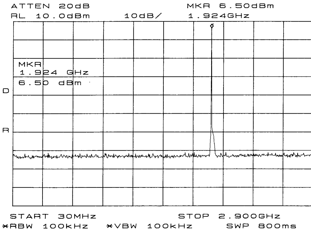
Figure 9: Emissions at Antenna Terminal.
