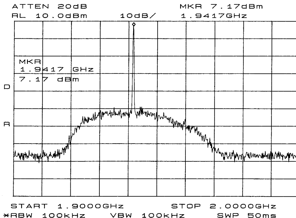
Figure 2: Downlink Power Output 1940.0 MHz.
