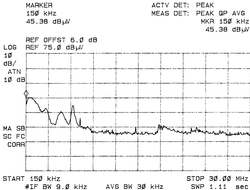
Figure 12: L1 line conducted emissions of EUT.
