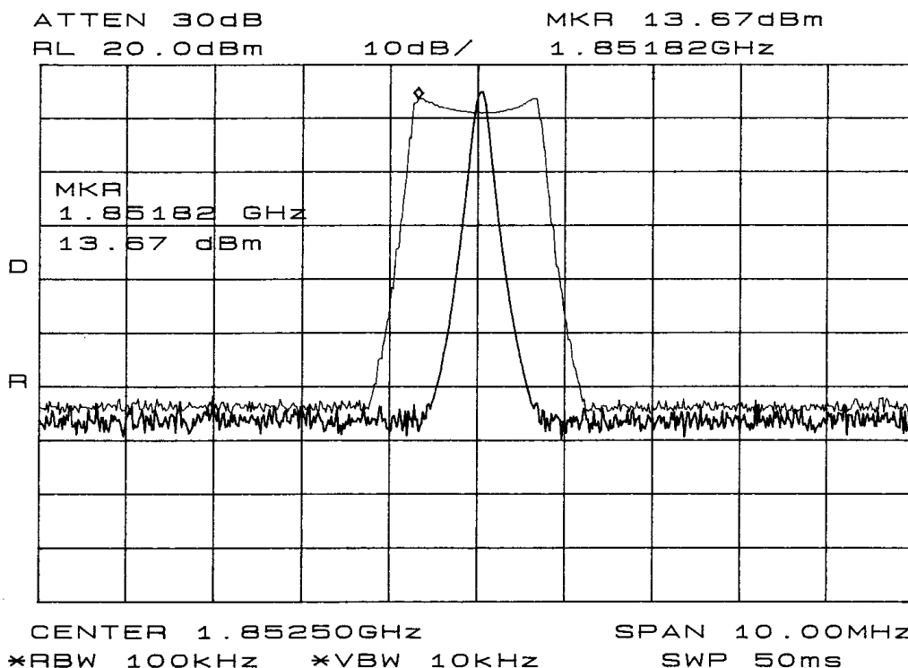
Figure 4: Occupied Bandwidth.
