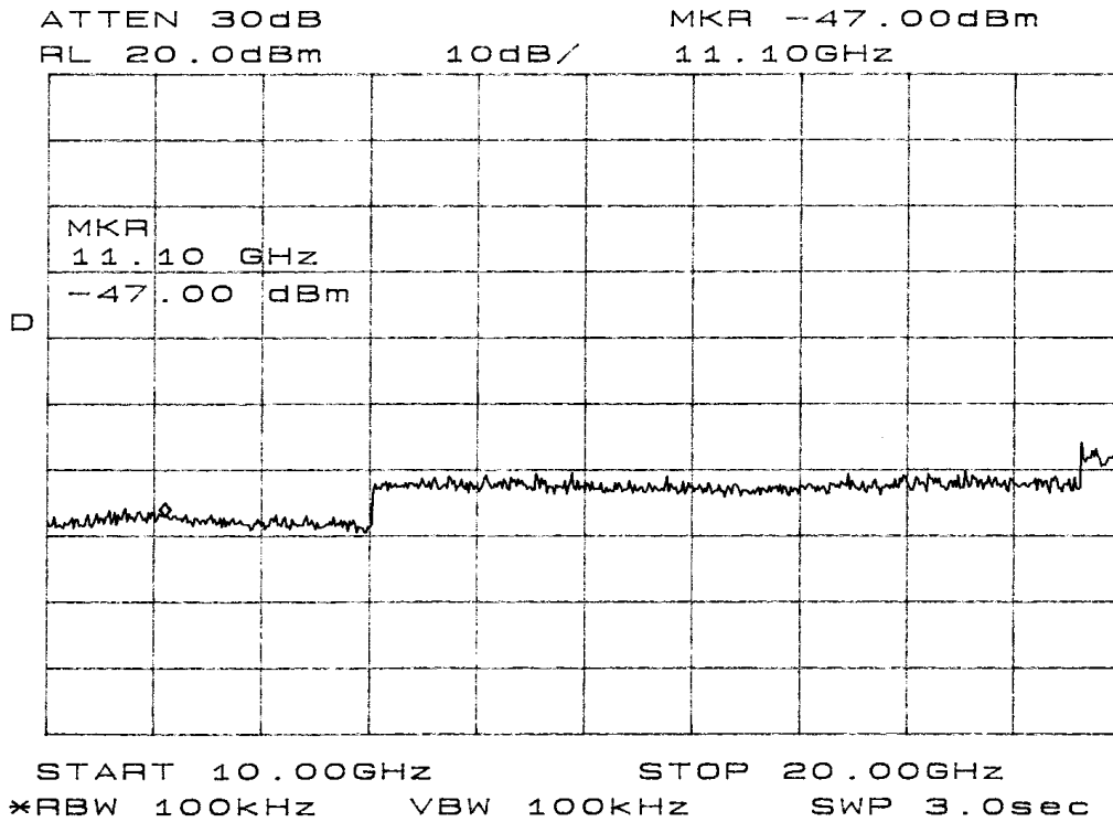
Figure 8: Emissions at Antenna Terminal.
