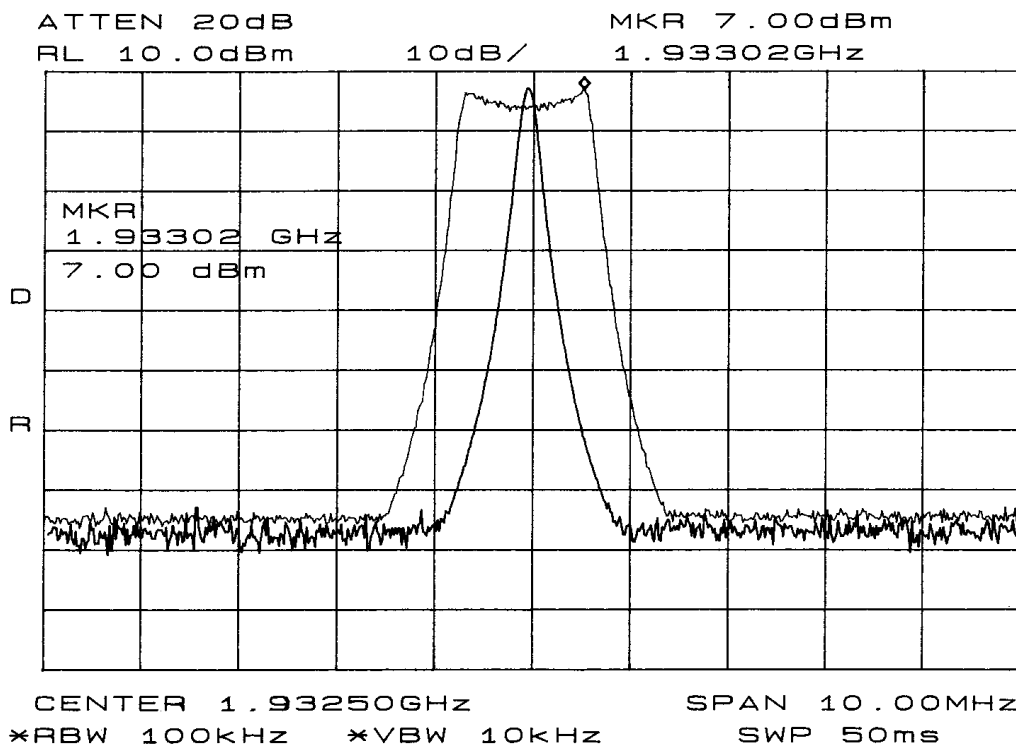
Figure 5: Occupied Bandwidth.
