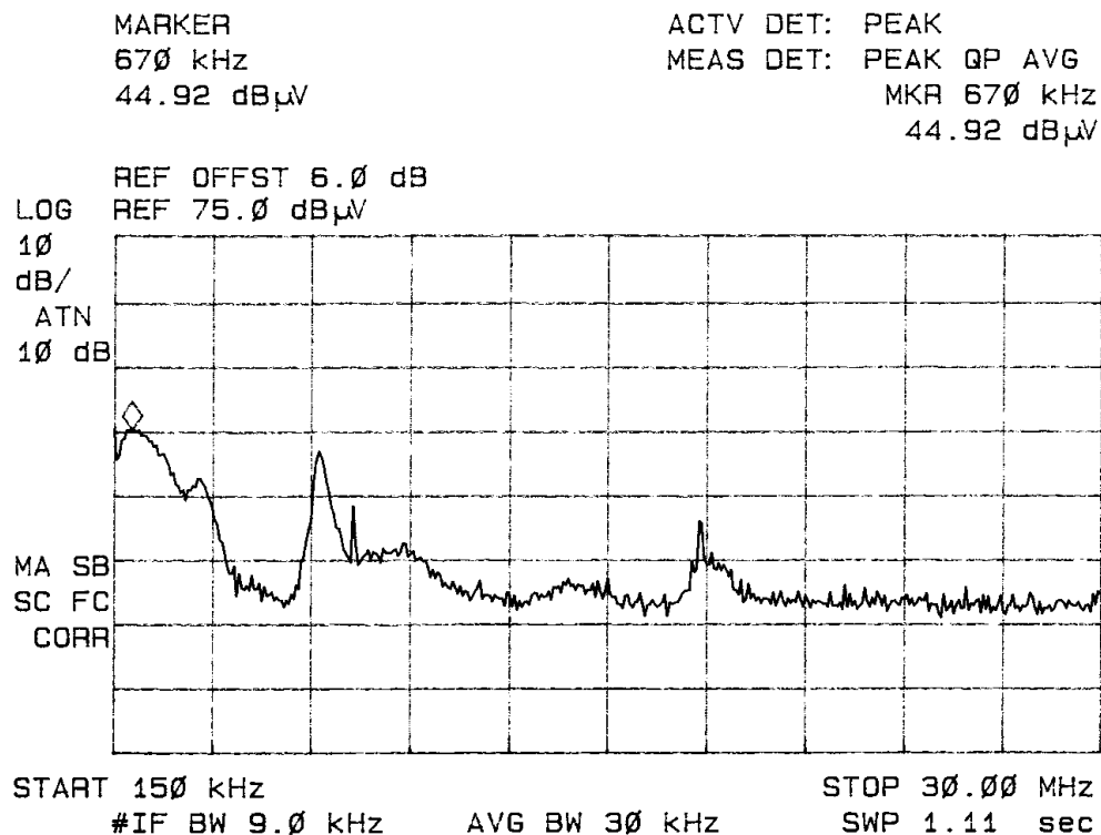
Figure 13: L2 line conducted emissions of EUT.
