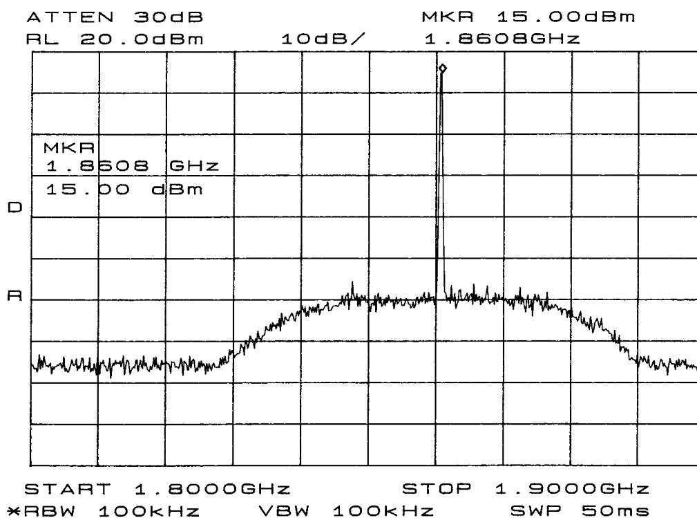
Figure 1: Uplink Power Output 1860.0 MHz.
