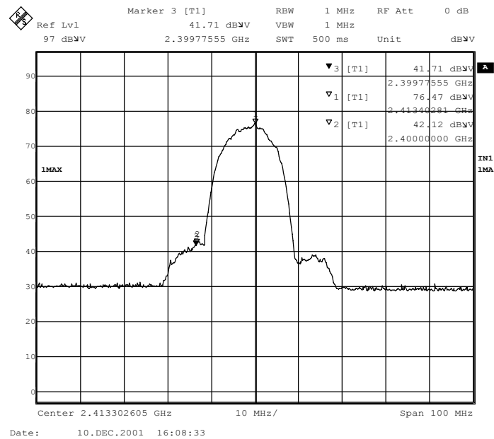
Figure Channel 1:11Mbps(Vertical)
