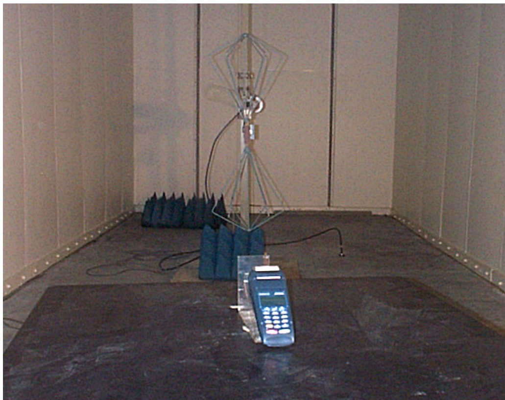
Spurious Emission Measurements of the device in the Frequency range 30 MHz-200 MHz
