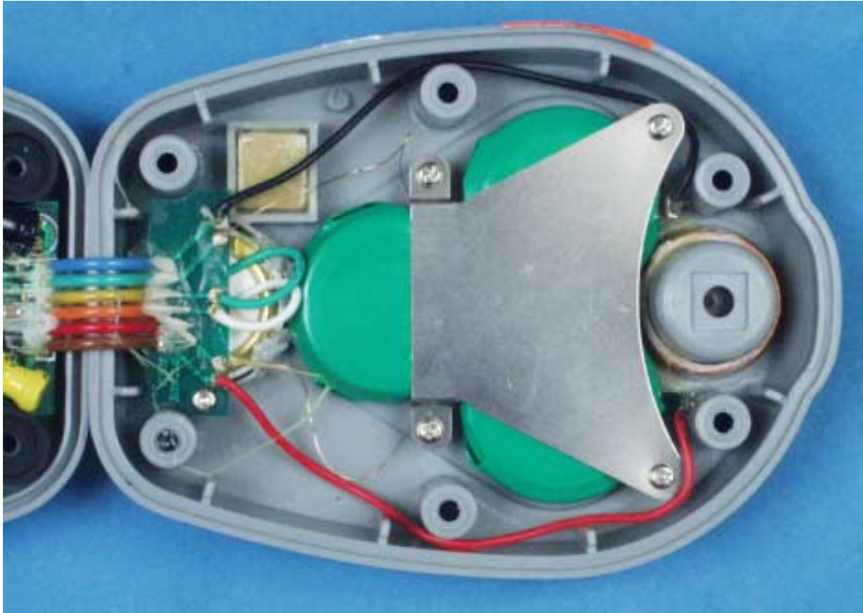
Inside Top Case
