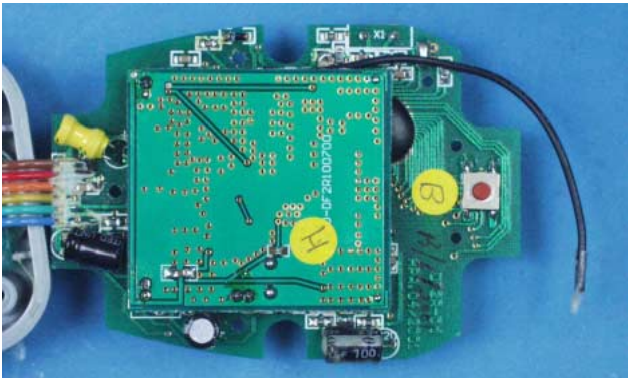
Regulator Board – Track Side
