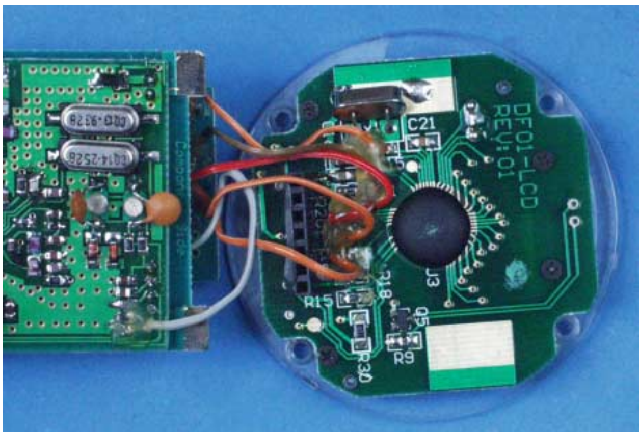
Panel Mount Display Board
