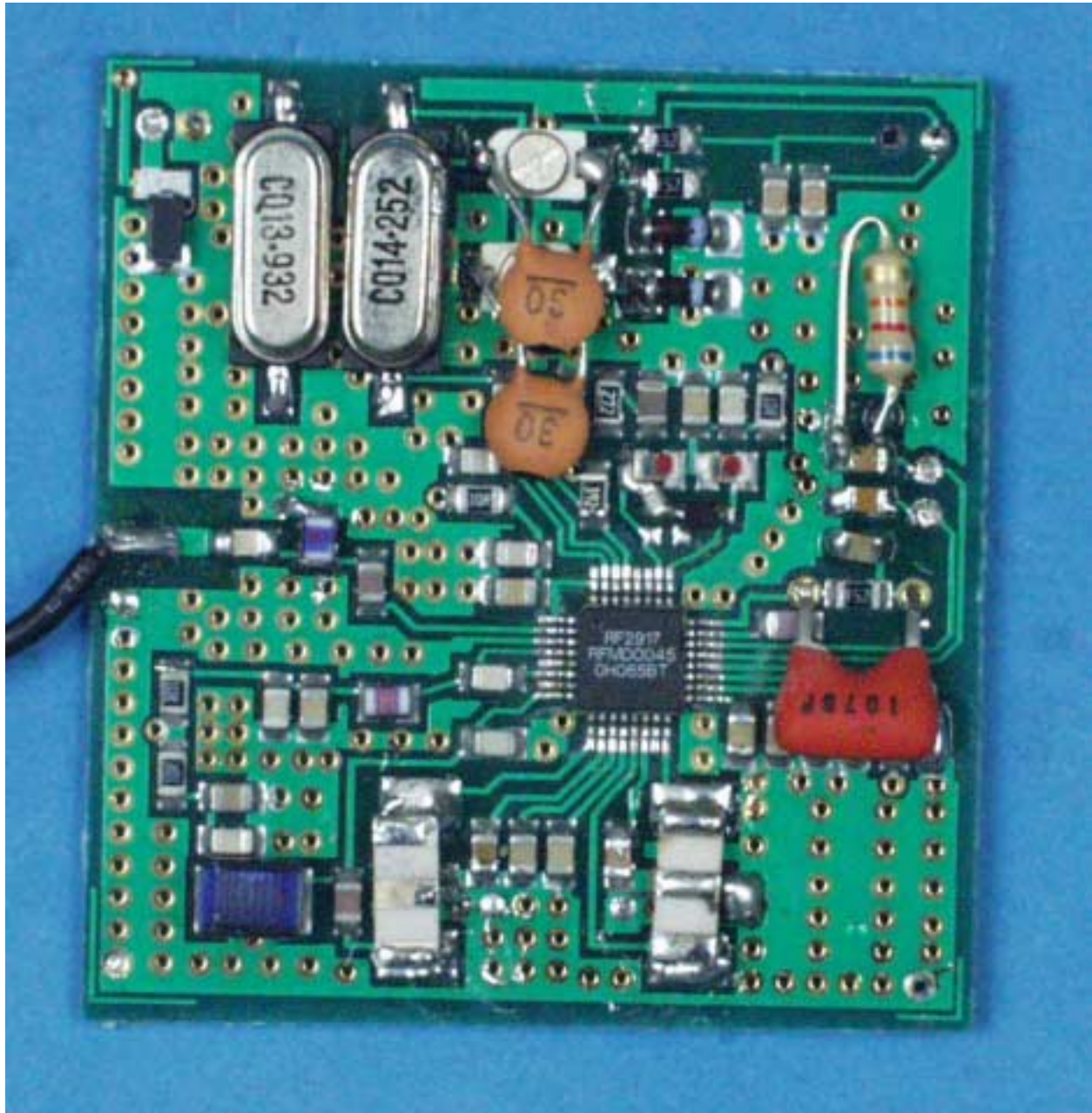
Common Receiver Board – Component Side
