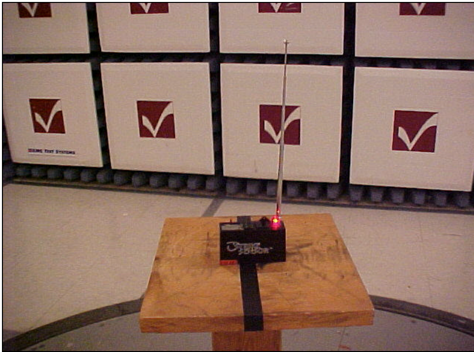
Front view of the Strike Sensor transmitter device during the radiated emissions tests.
