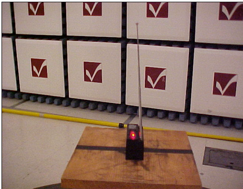
Rear view of the Strike Sensor transmitter device during the radiated emissions tests.
