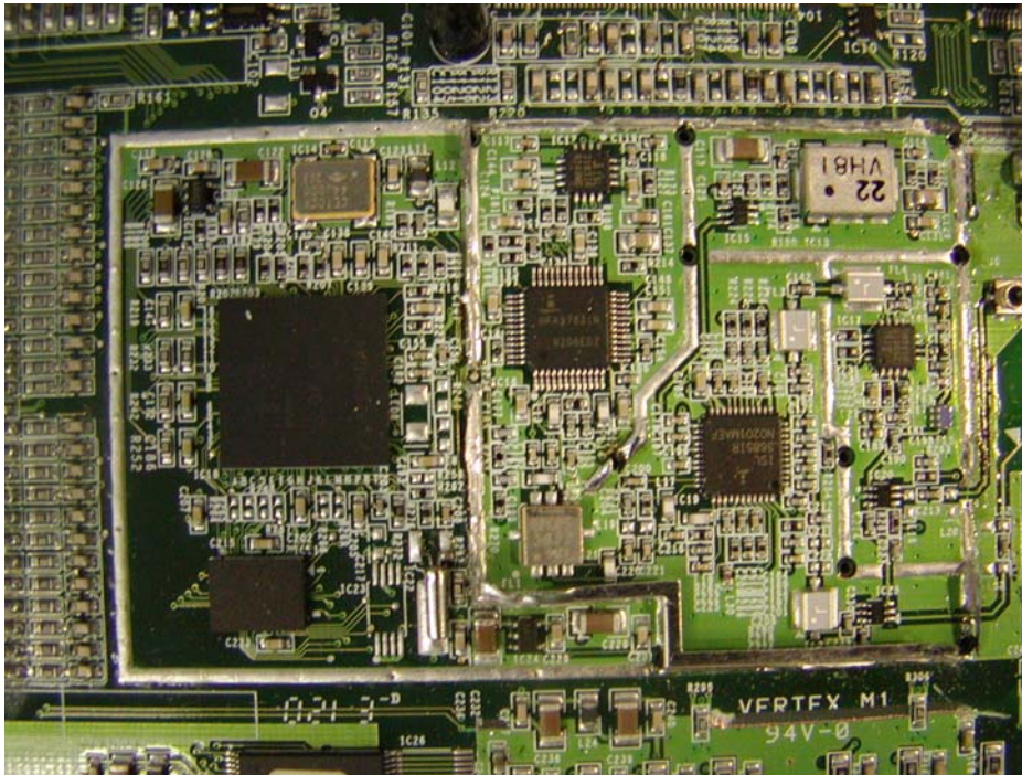
RF Board - Component View
