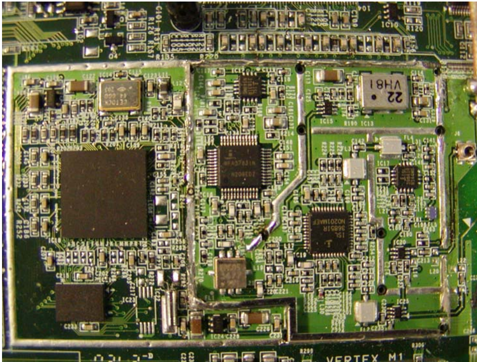
RF Board - Component View
