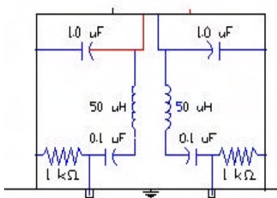
Figure 4. LISN Schematic Diagram
