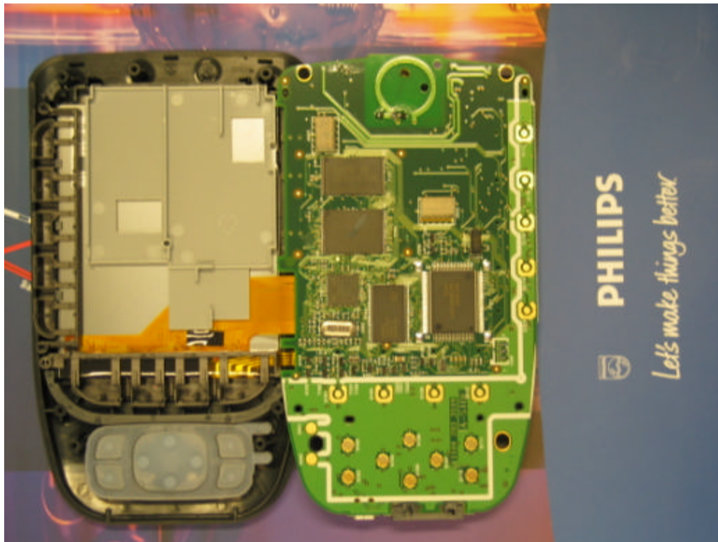
Figure 3: PWB TOP
