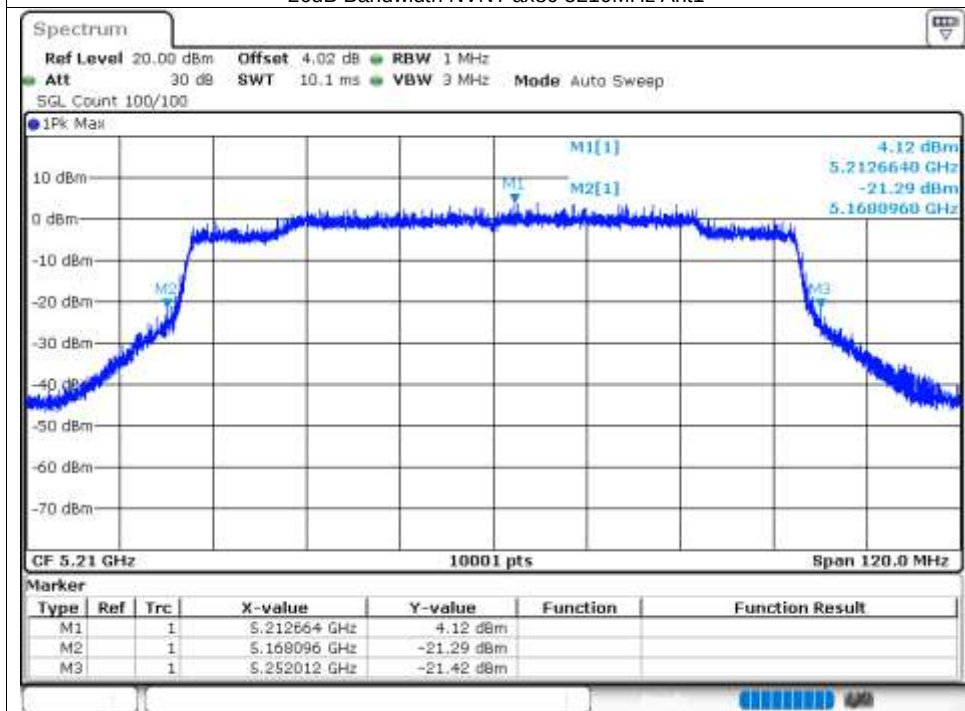
-26dB Bandwidth NVNT ax80 5210MHz Ant2
