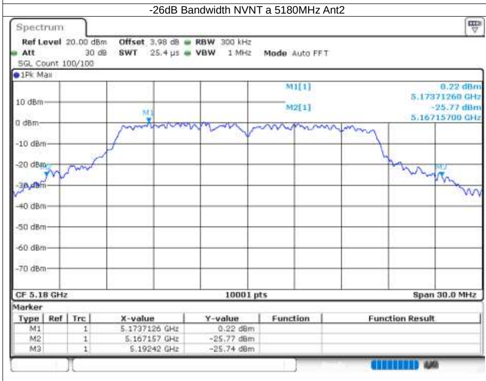
-26dB Bandwidth NVNT a 5180MHz Ant2
