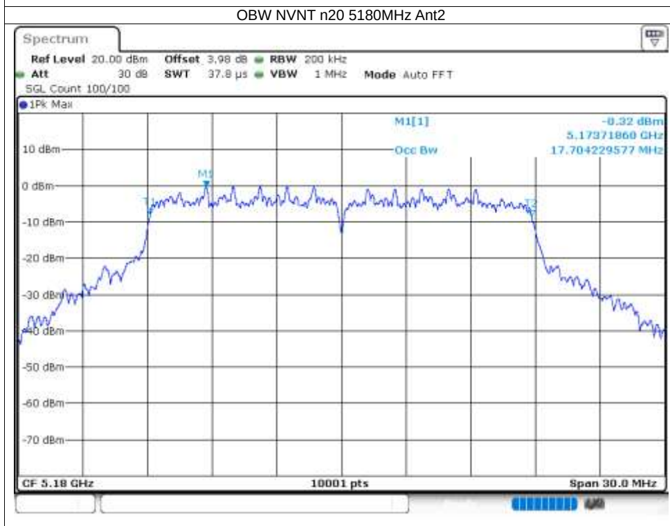
OBW NVNT n20 5180MHz Ant2
