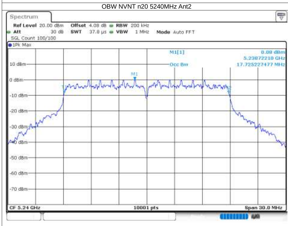
OBW NVNT n20 5240MHz Ant2
