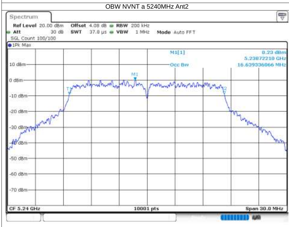
OBW NVNT a 5240MHz Ant2
