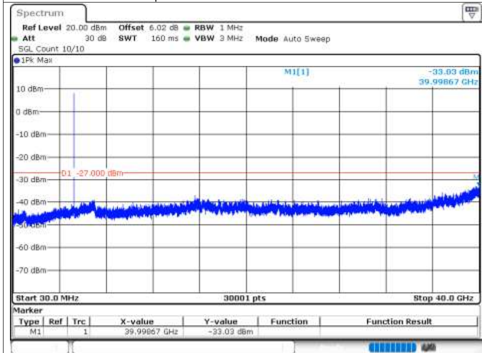
Tx. Spurious NVNT n20 5180MHz Ant2 Emission
