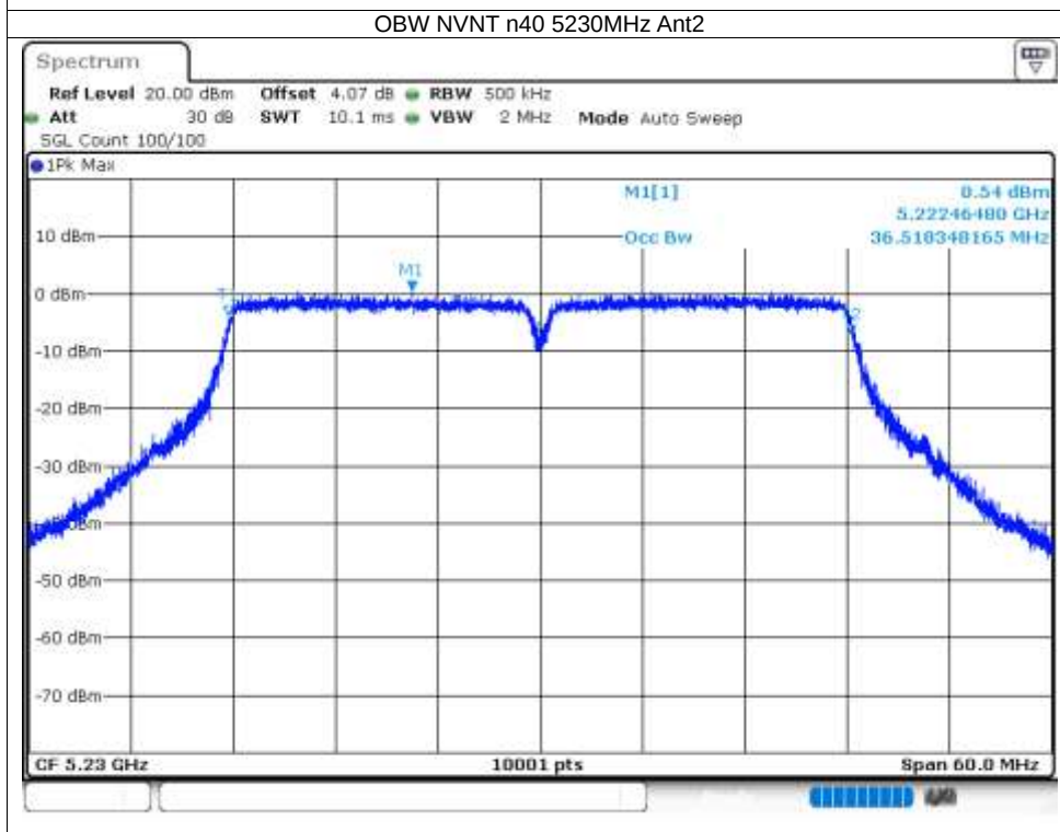
OBW NVNT n40 5230MHz Ant2
