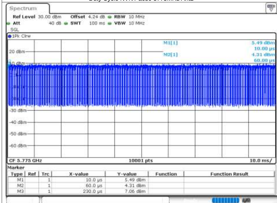
Duty Cycle NVNT ac80 5775MHz Ant2
