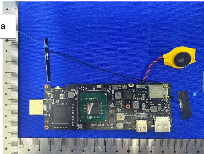
Secondary antenna
