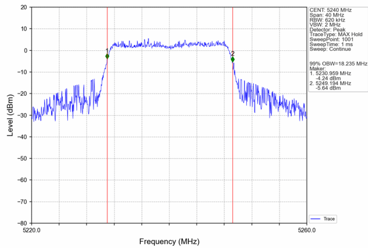
802.11n(HT20)_HCH_5240MHz_Ant2_NTNV
