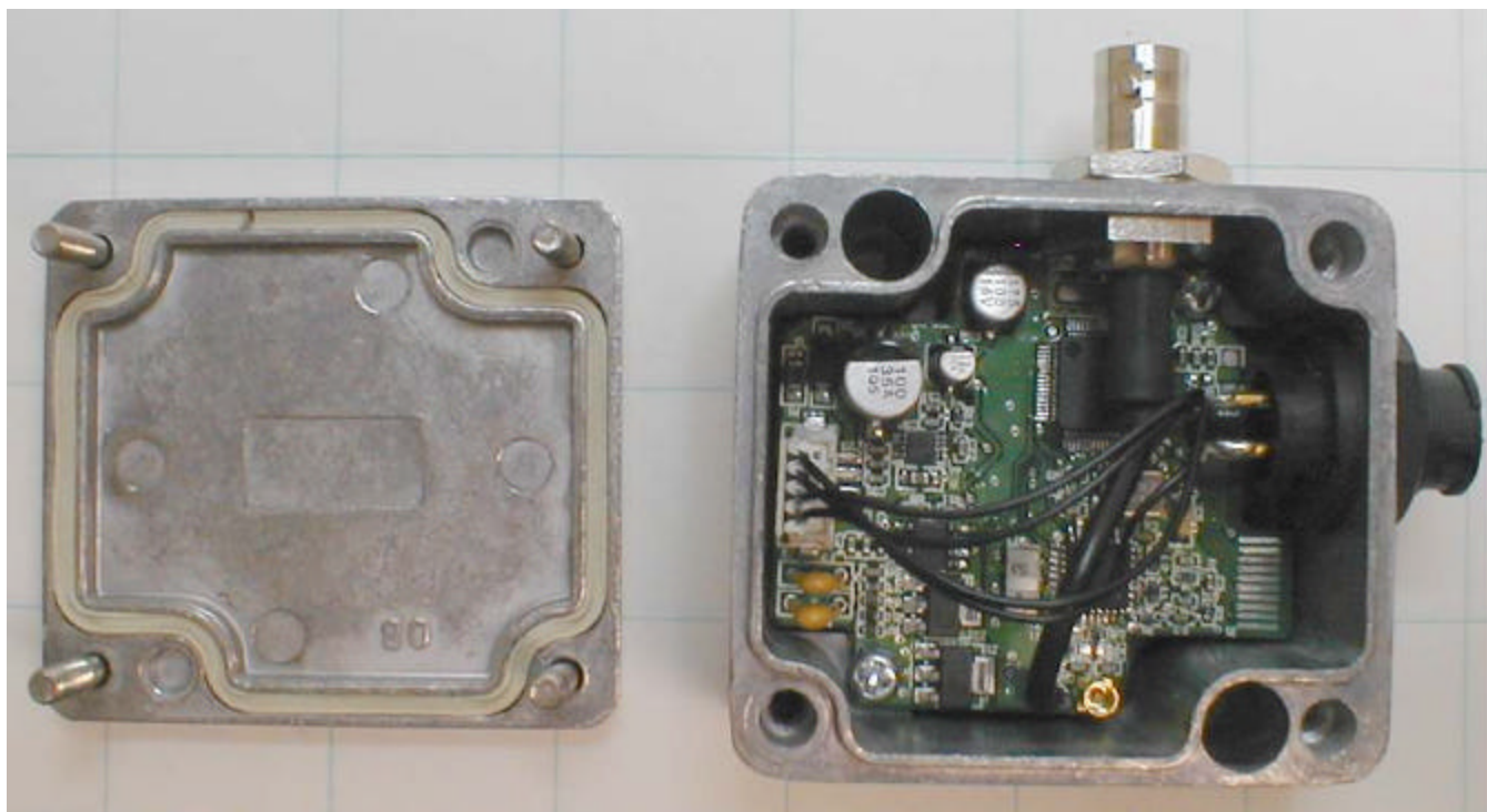
Link Cover Open
