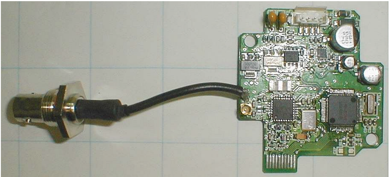
Link Radio Board Top
