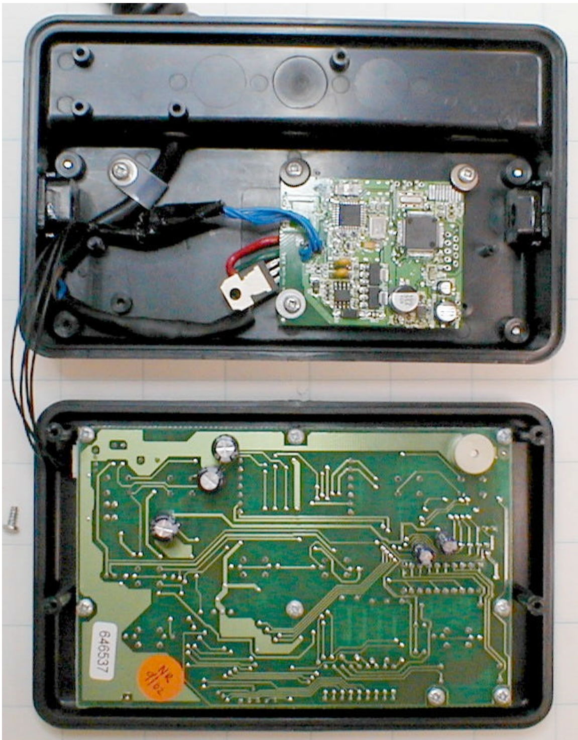
Remote Cover Open
