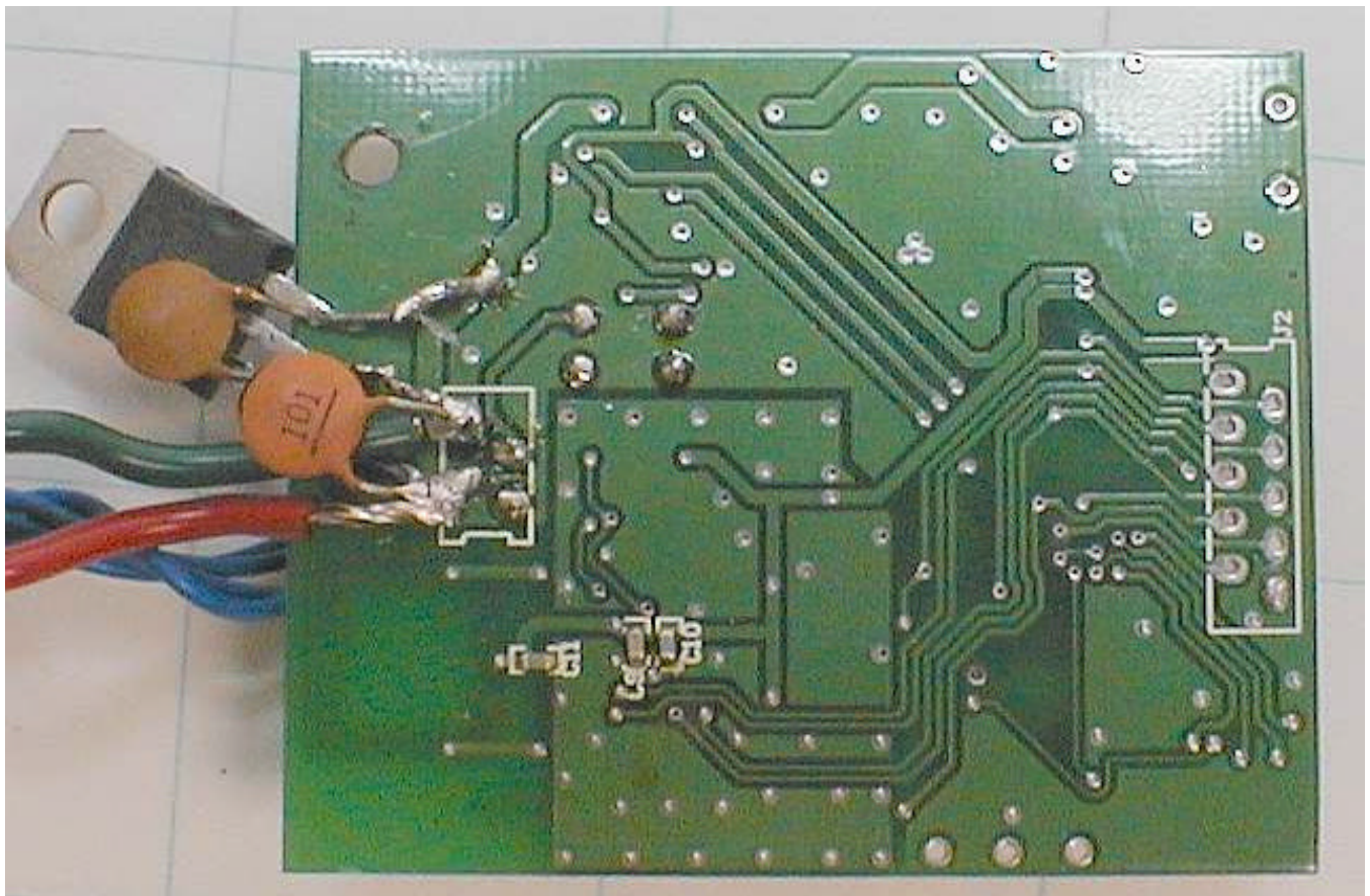
Remote Radio Board Bottom
