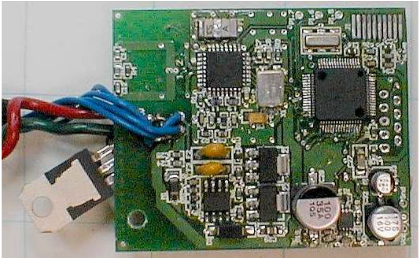
Remote Radio Board Top
