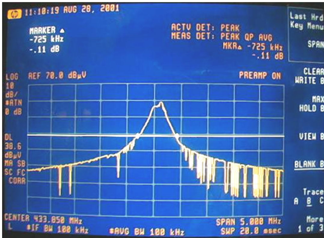
Fig 2. Receiver: Plot of the Transmitter Bandwidth Measurement
