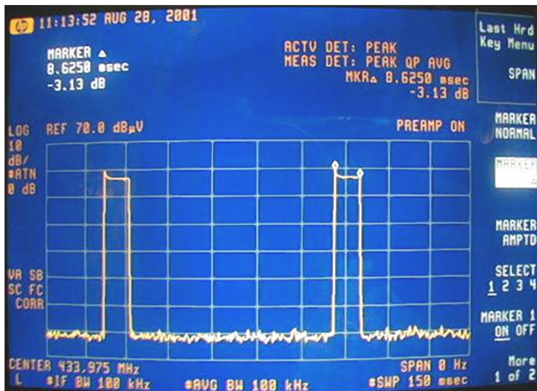
Fig 1. Receiver: Picture of the Duty Cycle Test
