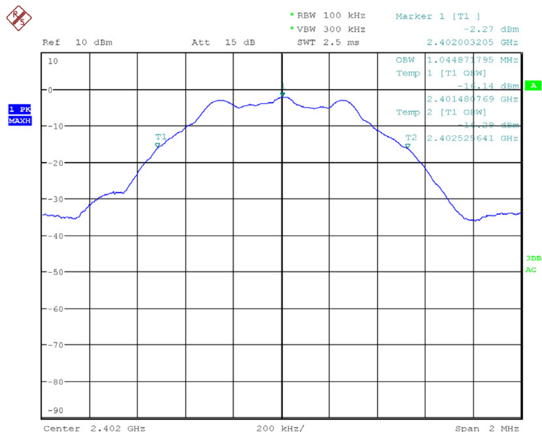
Graph 278: Occupied Bandwidth
