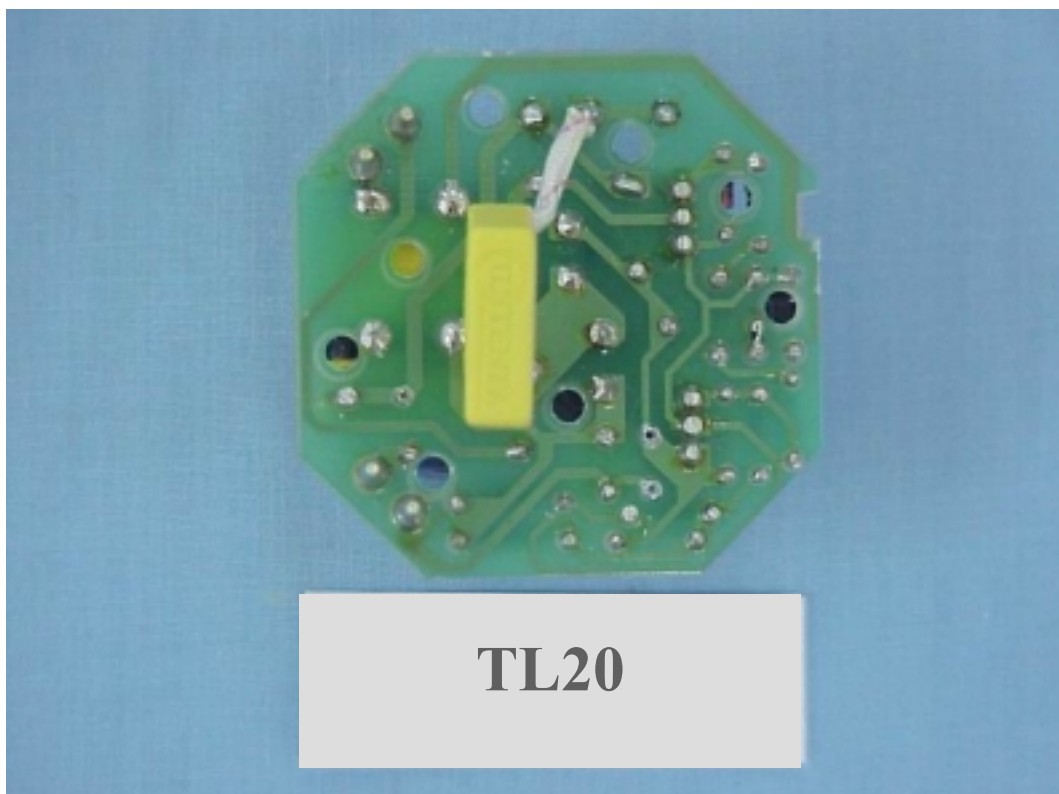
FIGURE 3 TWIST LAMP (M/N: TL20) MAIN BOARD (SOLDERED SIDE)
