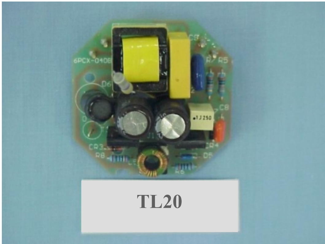
FIGURE 2 TWIST LAMP (M/N: TL20) MAIN BOARD (COMPONENT SIDE)
