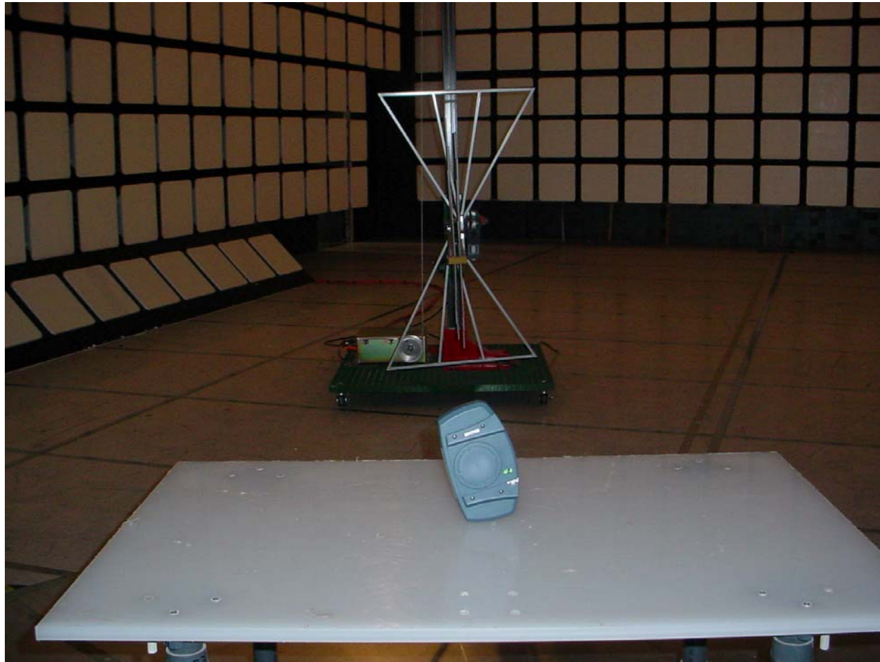
Photo #3: Radiated Emissions at 3 Meter Distance - The Model in.k707 was placed in position #3
