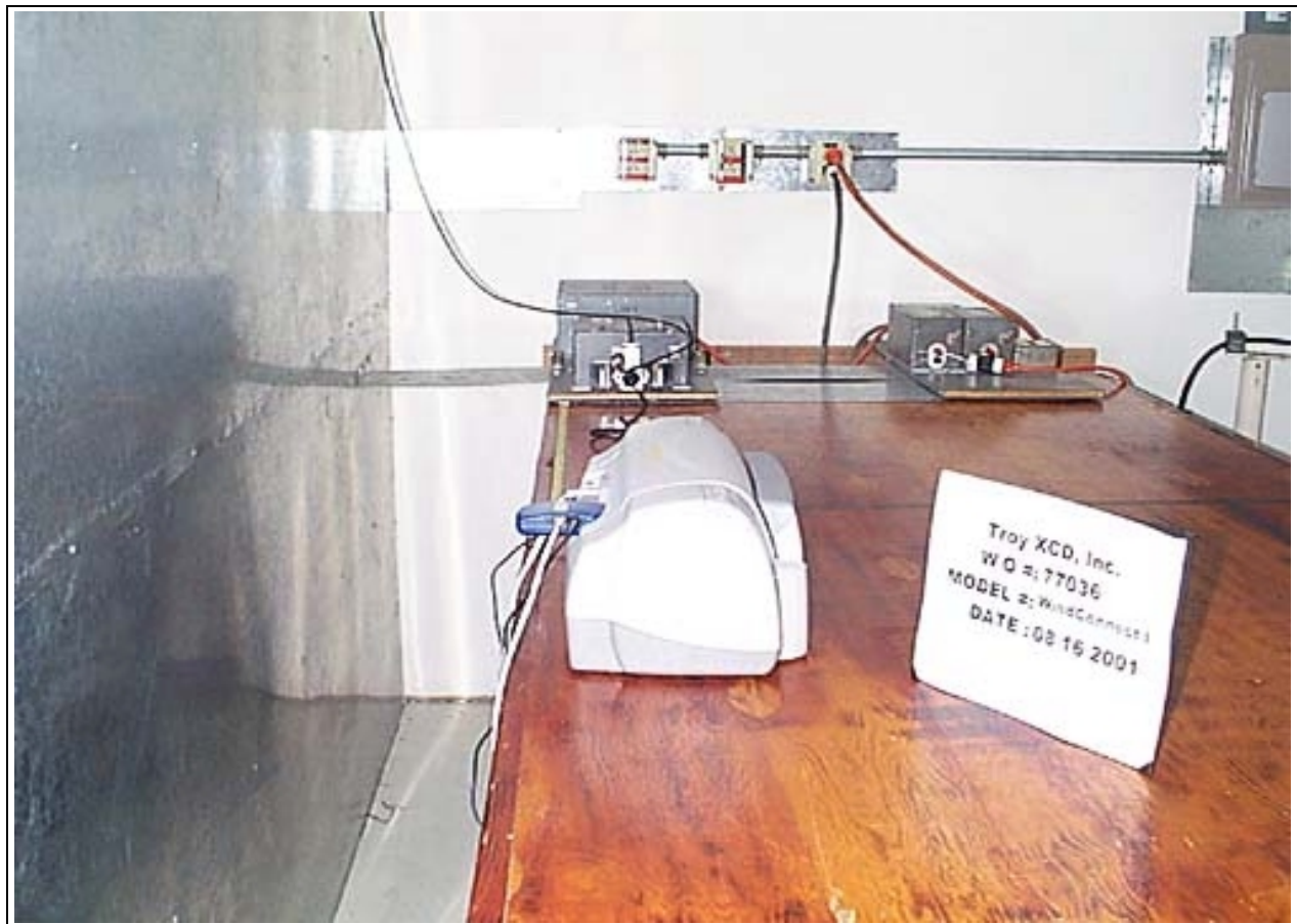
Mains Conducted Emissions - Back View (Brea Setup)
